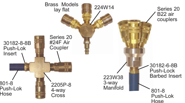
TYPICAL MANIFOLD APPLICATIONS
