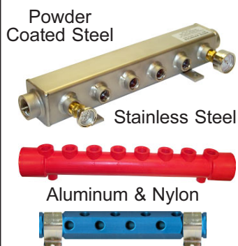
WATER MANIFOLDS
