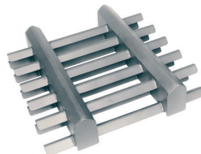
SUPER POWER GRATE MAGNET EASY-CLEAN DESIGN CERAMIC OR RARE EARTH
