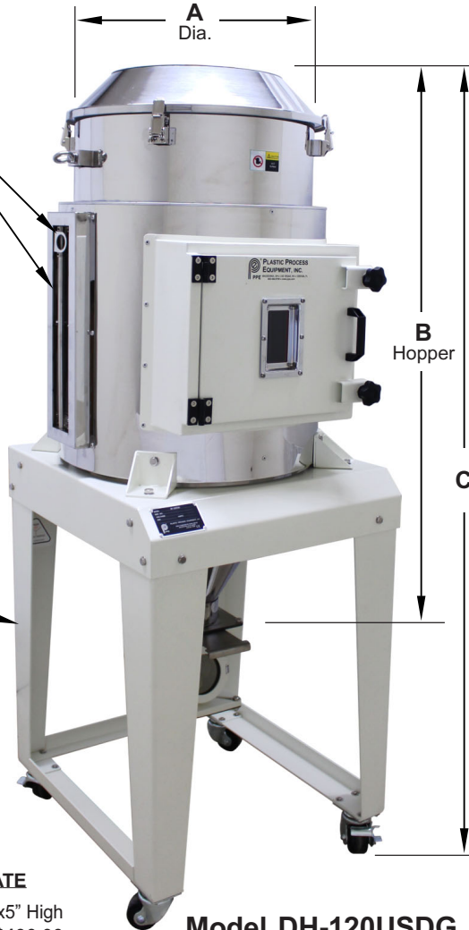
Model DH-120USDG Drying Hopper with stand and Cast Discharge Chute shown. 140lb. Capacity $1,705.00
