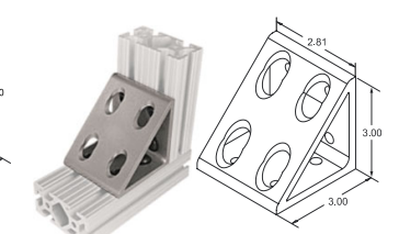
8 hole Inside Gusset Part No. EX4338 ..... $9.27
