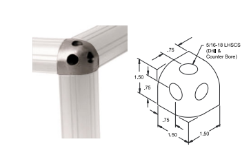
Rounded Tri-Corner Part No. EX4441 ..... $22.12
