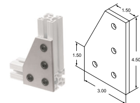
4 hole 90° Joining Plate Part No. EX4350 ..... $5.78
