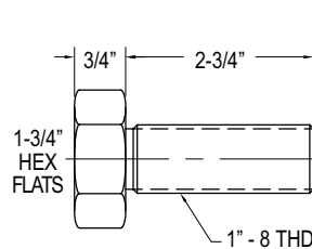
MODEL AB-2 HEEL ADJUSTMENT BOLT
