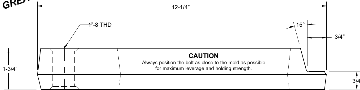
MODEL FCM-12 MOLD CLAMP
