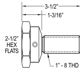
MODEL SAB1 SWIVEL HEEL ADJUSTMENT BOLT
