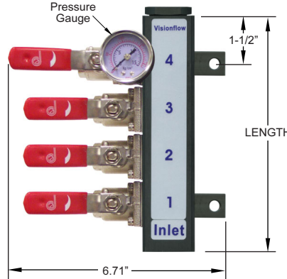
1" NPT at both ends (one end plugged)
