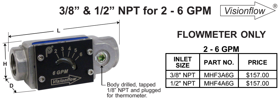
Dimensions 1.50" H x 1.77" D x 3.75" L
