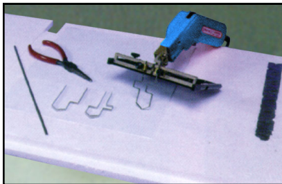
. . . and Bendable Blade Material.
