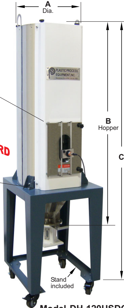
Model DH-120USDG Drying Hopper with standard Cast Discharge Chute shown. 140lb. Capacity
