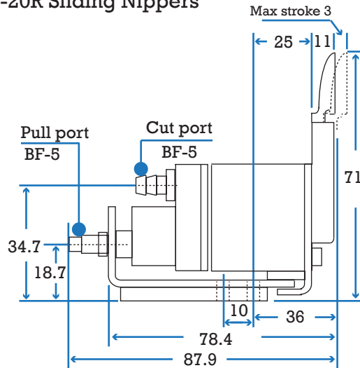
Position & mounting dimensions
