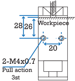
Position & mounting dimensions (QW-20)
