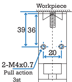
Position & mounting dimensions
