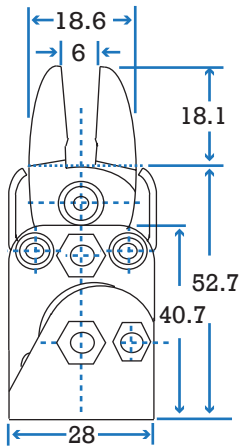
Position & mounting dimensions
