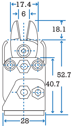
Position & mounting dimensions (QW-20)
