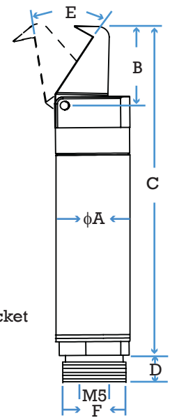
Sensor LM-9 (PNP or NPN)
