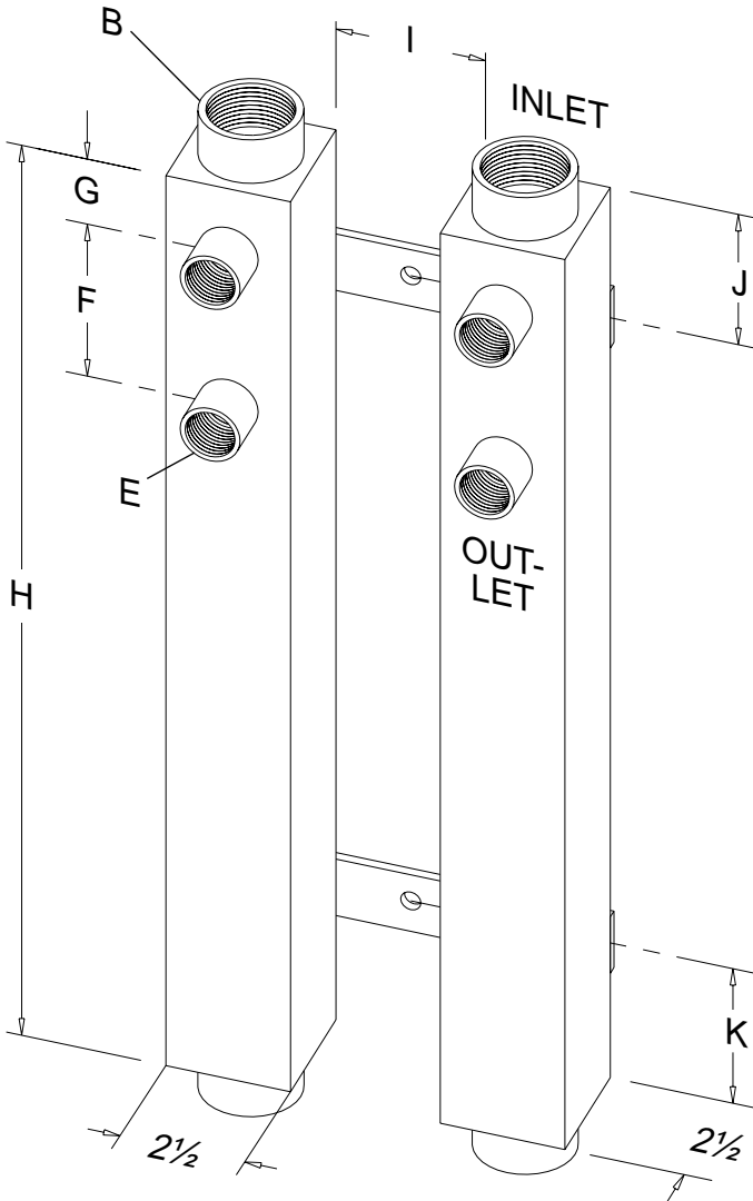
DUAL OUTLETS
